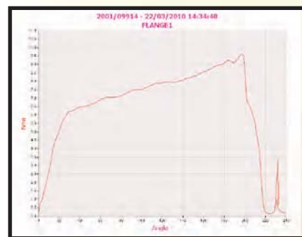
Torque vs Angle graph produced using T-Box MS software
